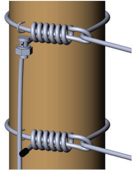
Staple Detail
