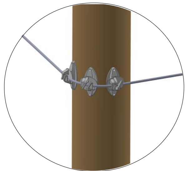
Typical Spacing for Raceline with Staples and Shockline with Insulators
