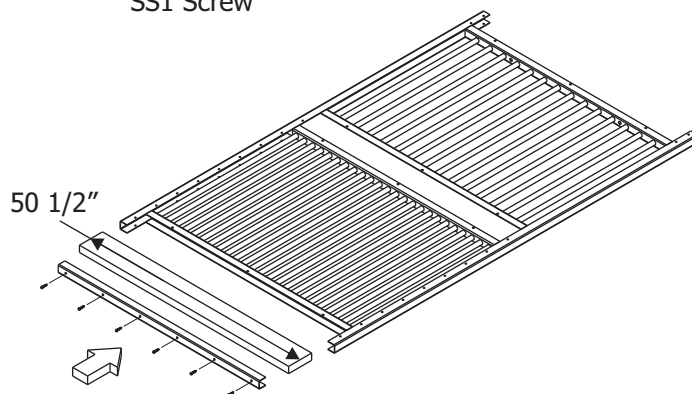
SS1 Screw
